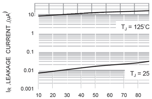
FIG.5-TYPICAL REVERSE CHARACTERIS
